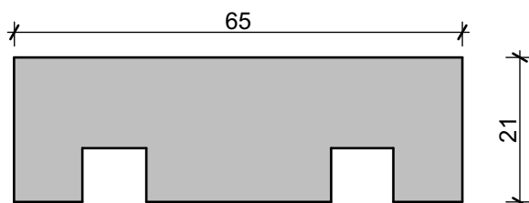
TNZ123 VERTICAL BATTEN
