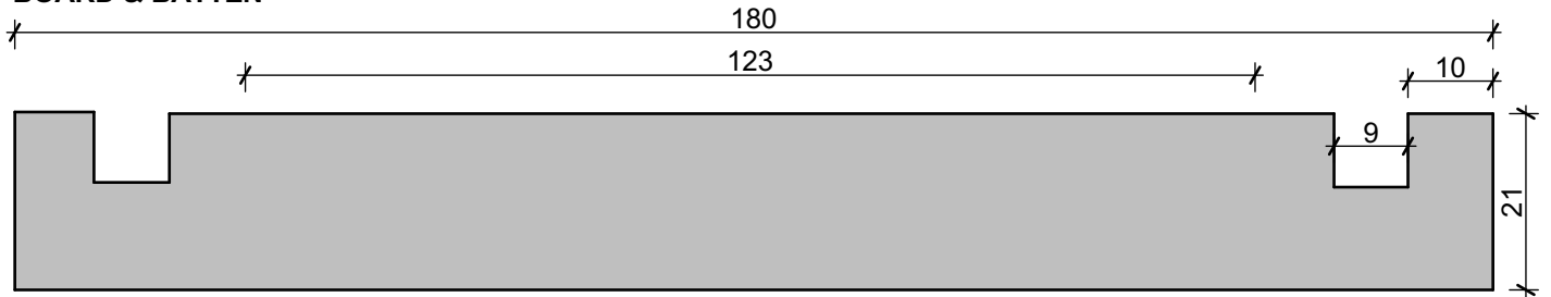
TNZ121 VERTICAL WEATHERBOARD
