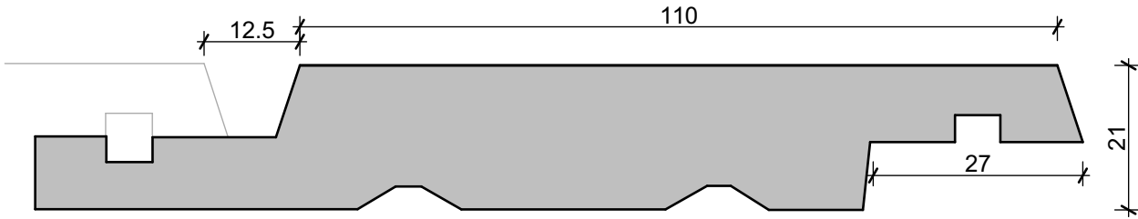
TNZ51 VERTICAL SHIPLAP
