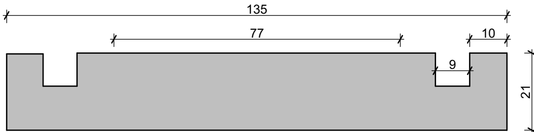
TNZ120 VERTICAL WEATHERBOARD
