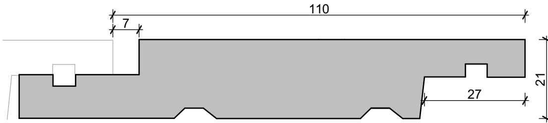
TNZ55 VERTICAL SHIPLAP
