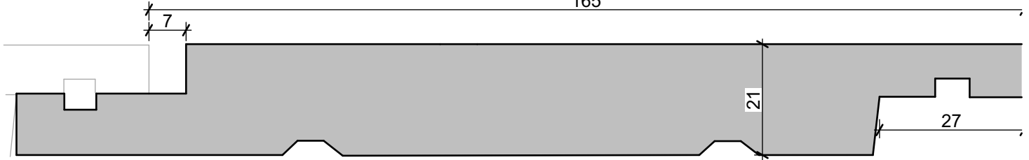
TNZ56 VERTICAL SHIPLAP -
