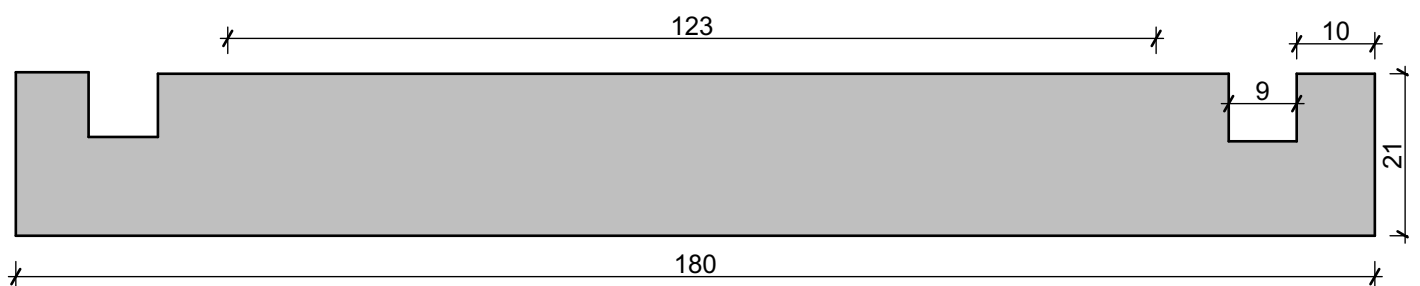
TNZ121 VERTICAL WEATHERBOARD
