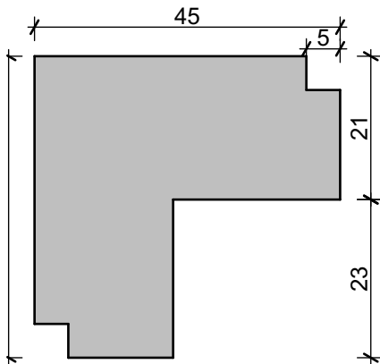
TNZ97 EXTERNAL CORNER
