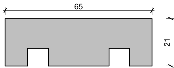
TNZ123 VERTICAL BATTEN
