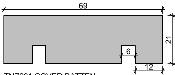
TNZ201 COVER BATTEN
