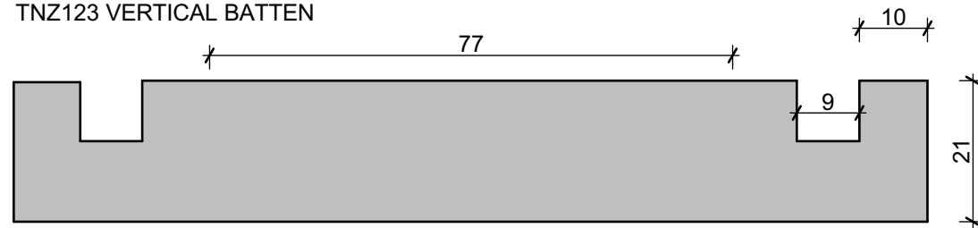
TNZ120 VERTICAL WEATHERBOARD
