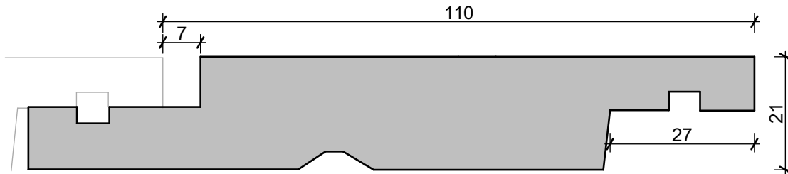
TNZ55 VERTICAL SHIPLAP -
