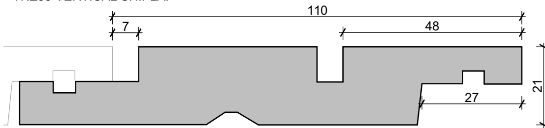
TNZ58 VERTICAL SHIPLAP -*CLEARS ONLY
